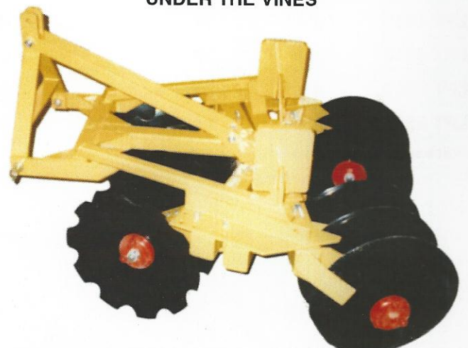
VIEW SHOWING MASSIVE CONSTRUCTION AND THE QUICK AND EASY ADJUSTMENTS OR WIDTH AND ANGLE SETTING
